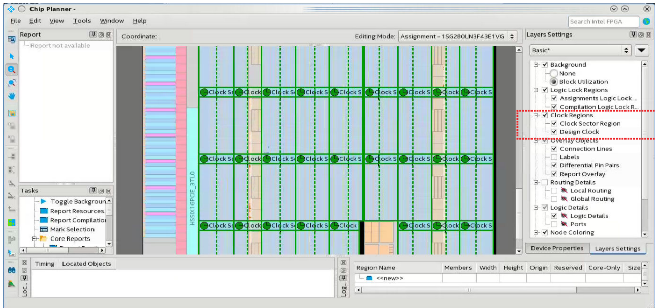
Figure 34. Clock Regions
